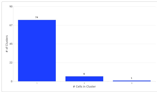
Cluster Size
